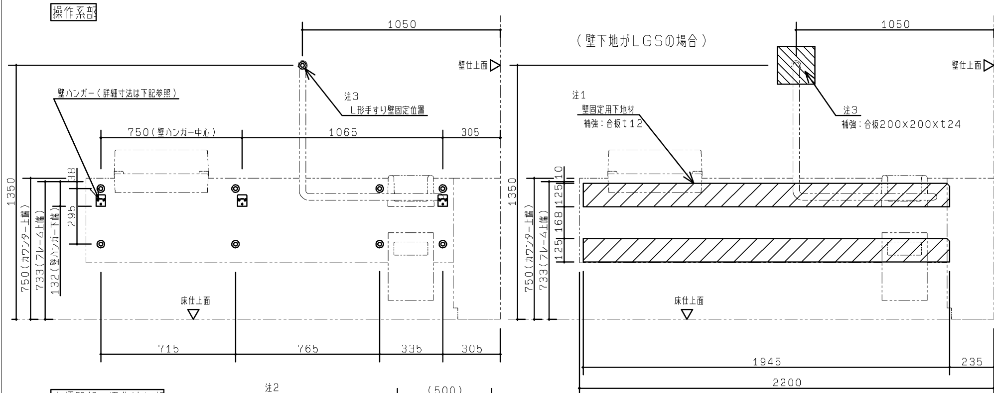
壁ハシガ一部詳細 ( S = 1 / 4 )
