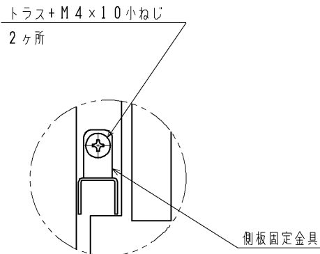
B部詳細 (S=1:2)
