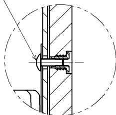
C部詳細 (S=1:2)
