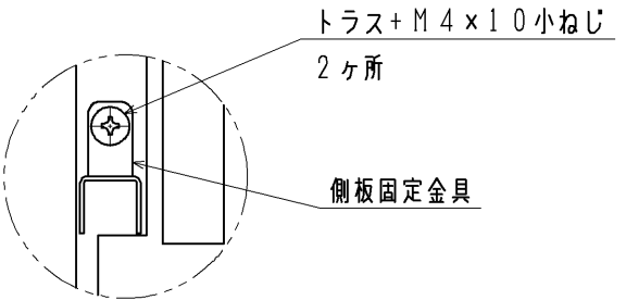
B部詳細 (S=1:2)
