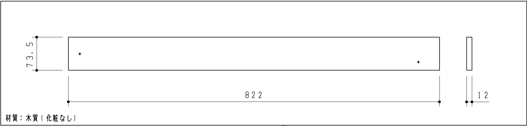
下段補強桟
