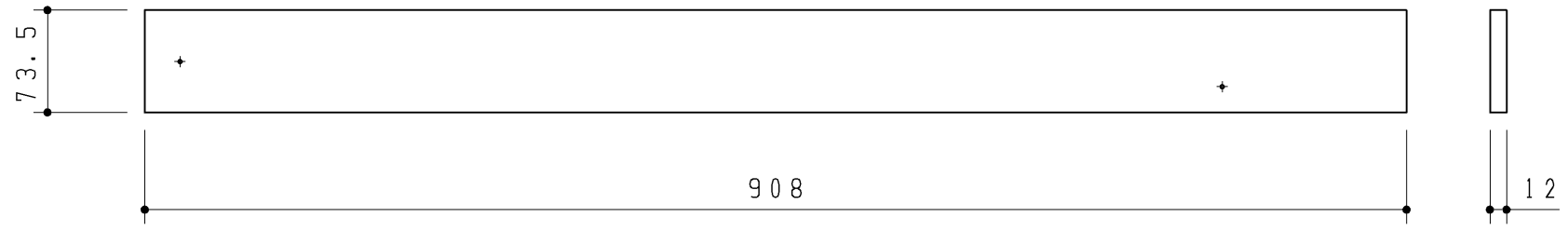
下段補強桟
