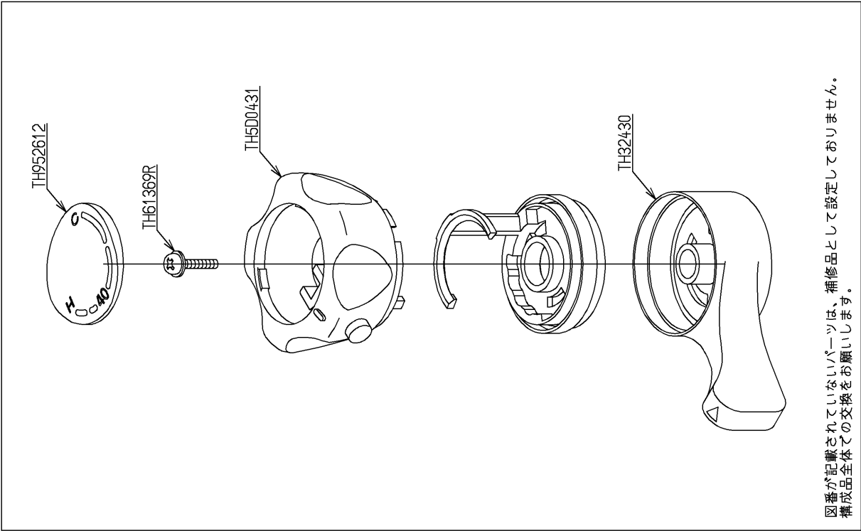
[分解図]
